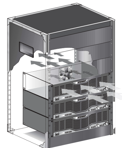
Figure 2.2 Airflow
