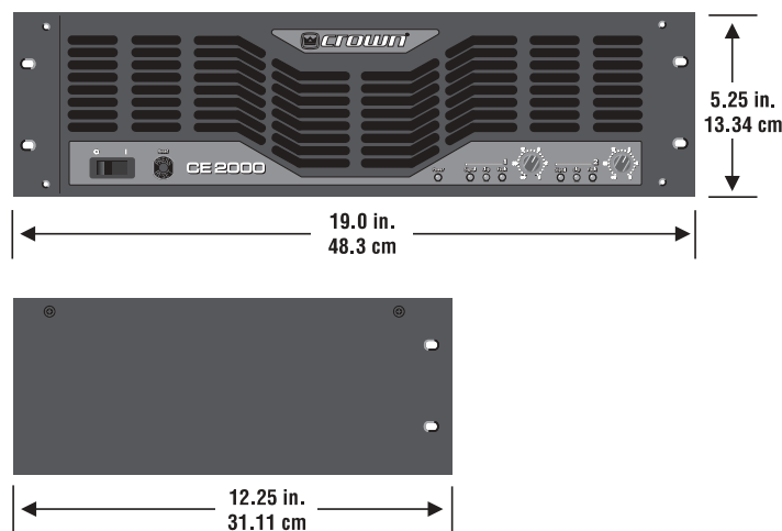
Figure 2.1 CE 1000 and CE 2000 Dimensions
