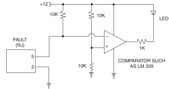
Figure 4.4 Fault Status LED Circuitry
