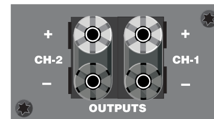
Figure 4.7 Model CEAS2 5-way Binding Post Output Connectors
