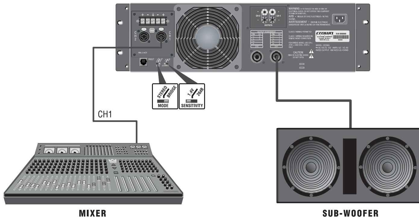
Figure 2.11 Typical System Wiring, Bridge-Mono Mode
