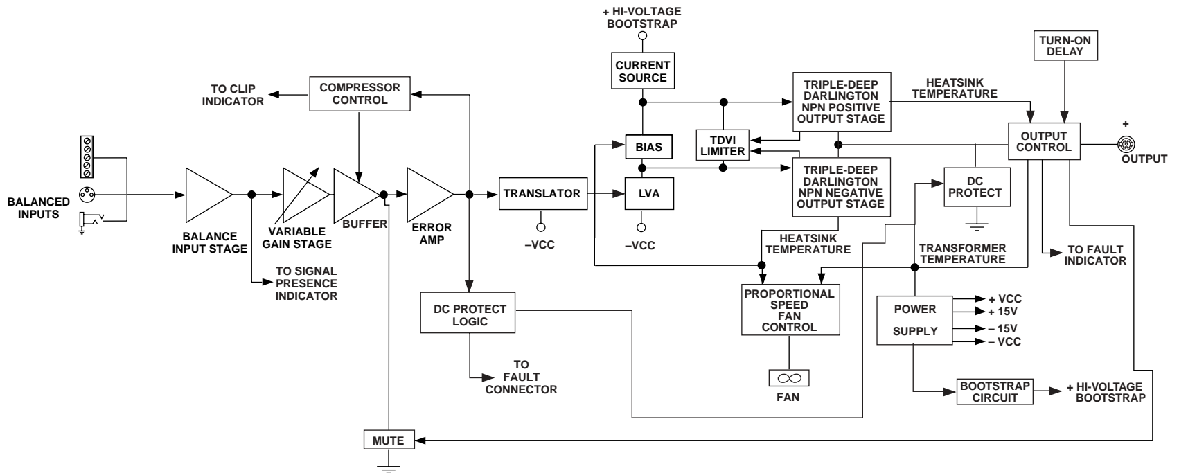
Figure 5.1 CE Series Amplifier Block Diagram (Shown with Standard Input Module)
