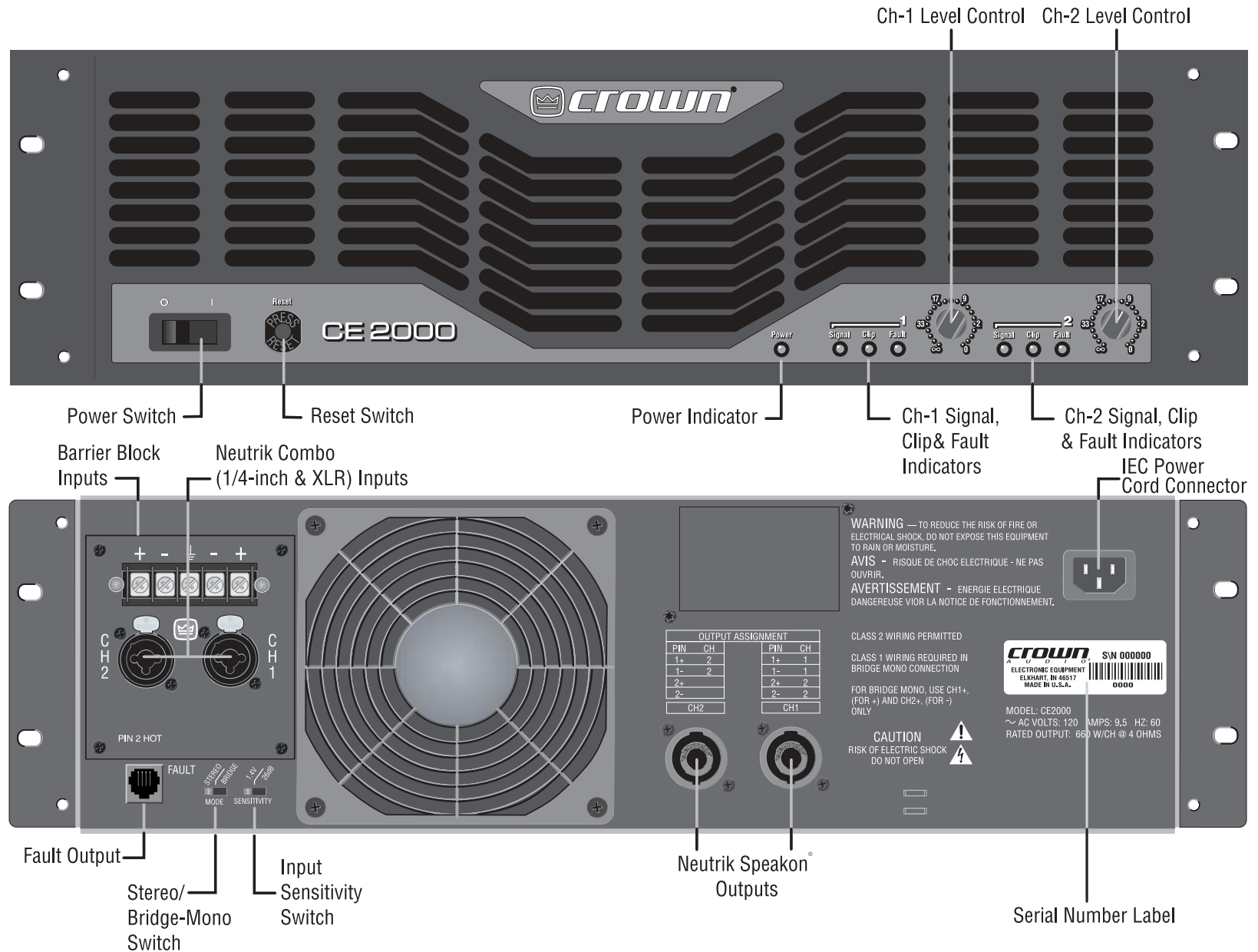
Figure 3.1 Controls, Indicators & Connectors
