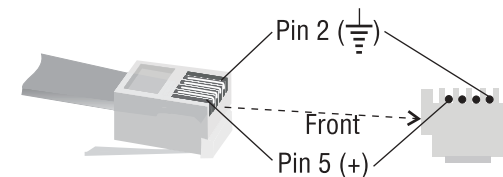
Figure 4.5 RJ-11 Jack Wiring and Pin Assignments
